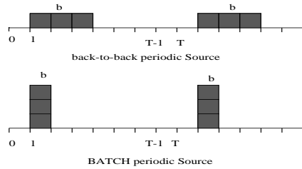
Figure 1 Back-to-back and Batch periodic sources.
