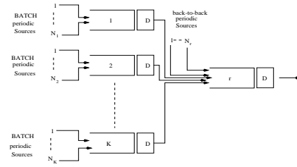
Figure 2 Two-stage tree network.
