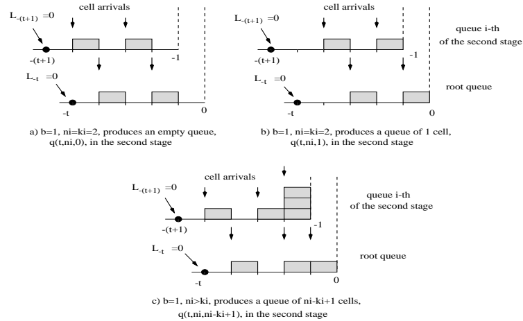
Figure 3 Cases to calculate the term R^{n_i}(t, k_i, n_i) , (with b=1 ).
